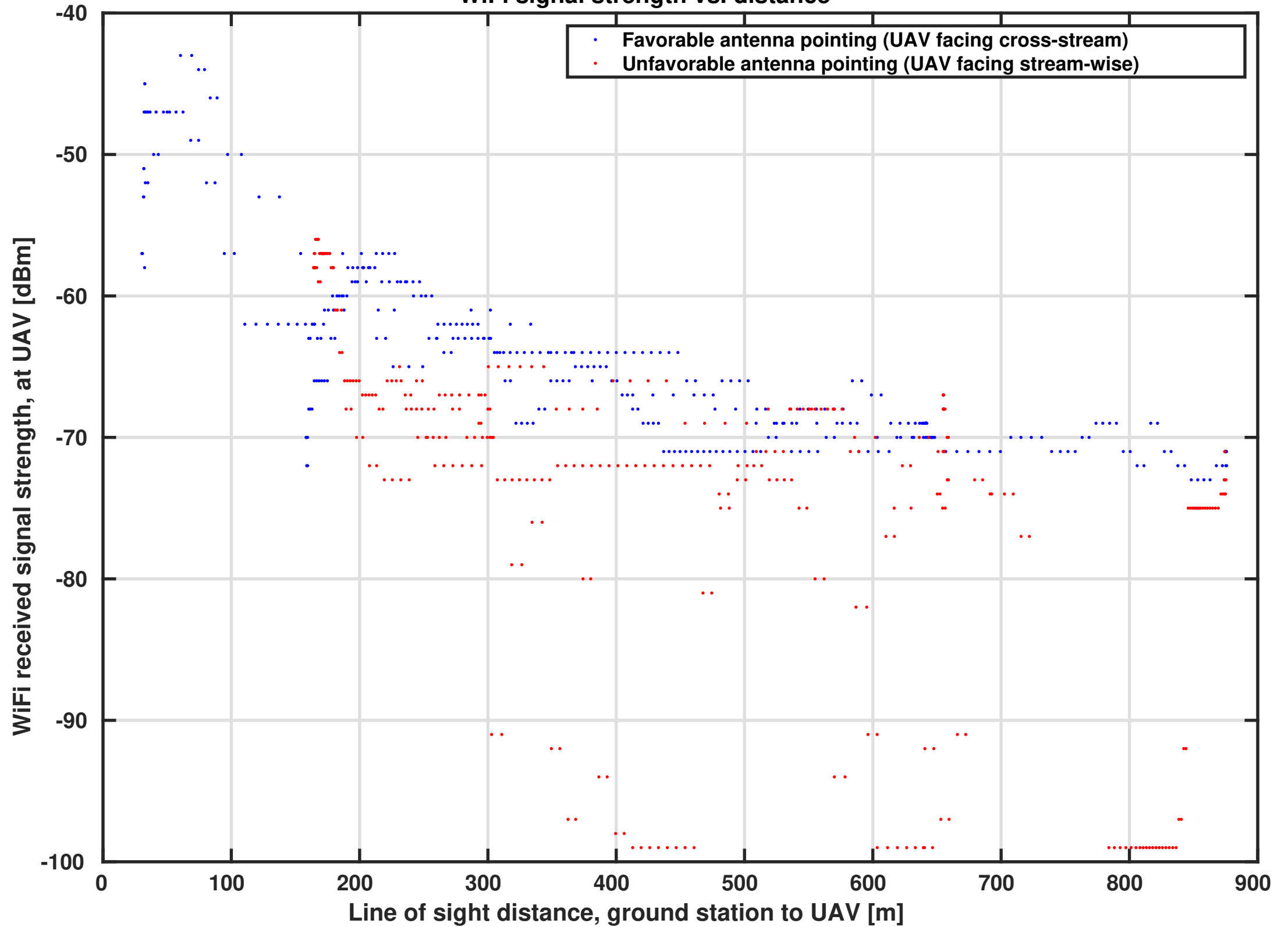
WiFi signal strength vs. distance
